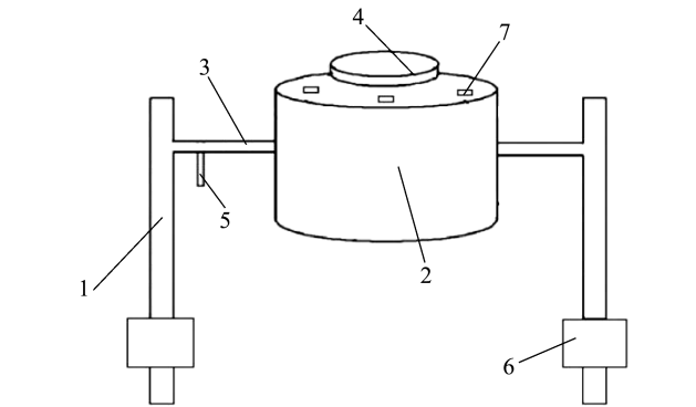
Fig.1 Microwave drying apparatus explanatory note: 1. Support frame; 2. drying box; 3. spindle; 4.material cover; 5.connection shaft; 6.axis of activity; 7.microwave generator.
