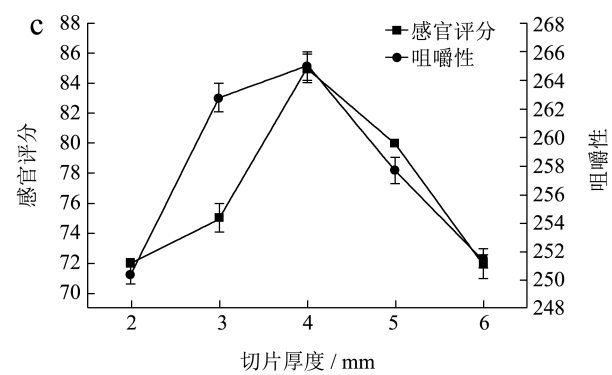
图 5 黄瓜钱儿微波干燥脱水工艺单因素试验结果 Fig.5 Results of single factor experiment on microwave drying and dehydration process of dried cucumber slices
