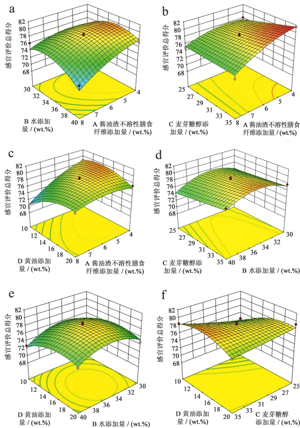
图 5 任意 2 个因素交互作用对感官评价总得分影响的响应面图 Fig.5 Response surface diagram of the impact of interaction of any two factors on the total score of sensory evaluation
