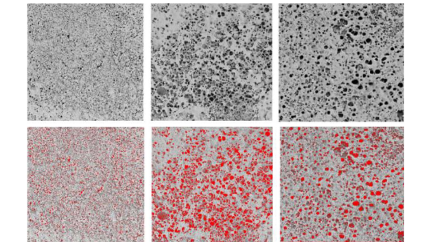
图 1 部分样品的孔隙率测定结果 Fig.1 Porosity measurement results of some samples
