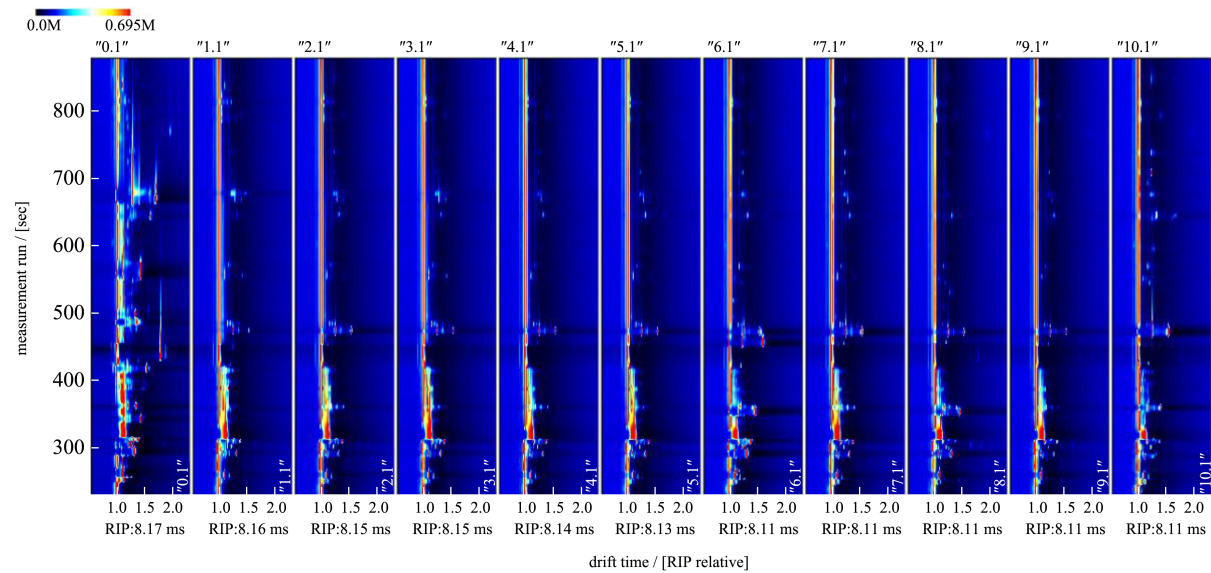
图 2 样品的 GC-IMS 二维谱图比较 Fig.2 Comparison of gc-ims two-dimensional spectra of samples
