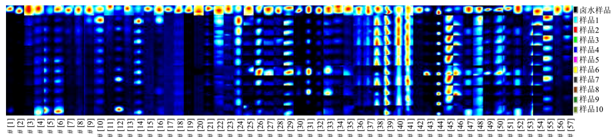
图 3 样品挥发性风味物质指纹图谱 Fig.3 Fingerprint of volatile flavor compounds in the sample
